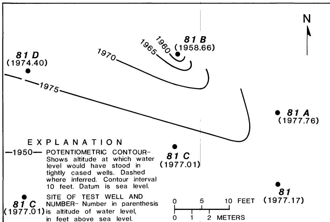
Figure 7.—Equipotential lines in bedrock above coal after 70 minutes of pumping well 81B at 1.1 gallons per minute.
