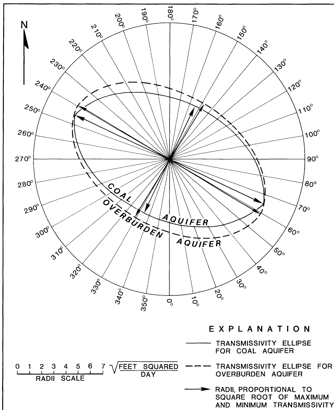
Figure 10.—Least-squares transmissivity ellipses for coal and overburden aquifers for aquifer tests December 10 and 17, 1981, Preston County, West Virginia.
