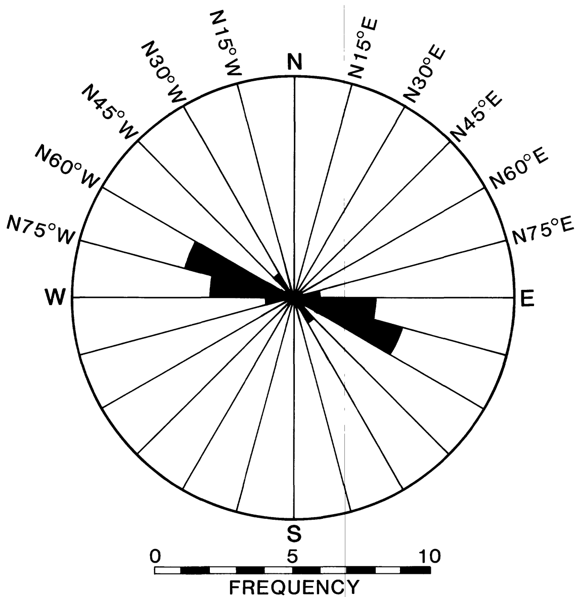
Figure 9.—Rose diagram showing frequency of orientation of the major component of transmissivity in Upper Freeport coal aquifer.
