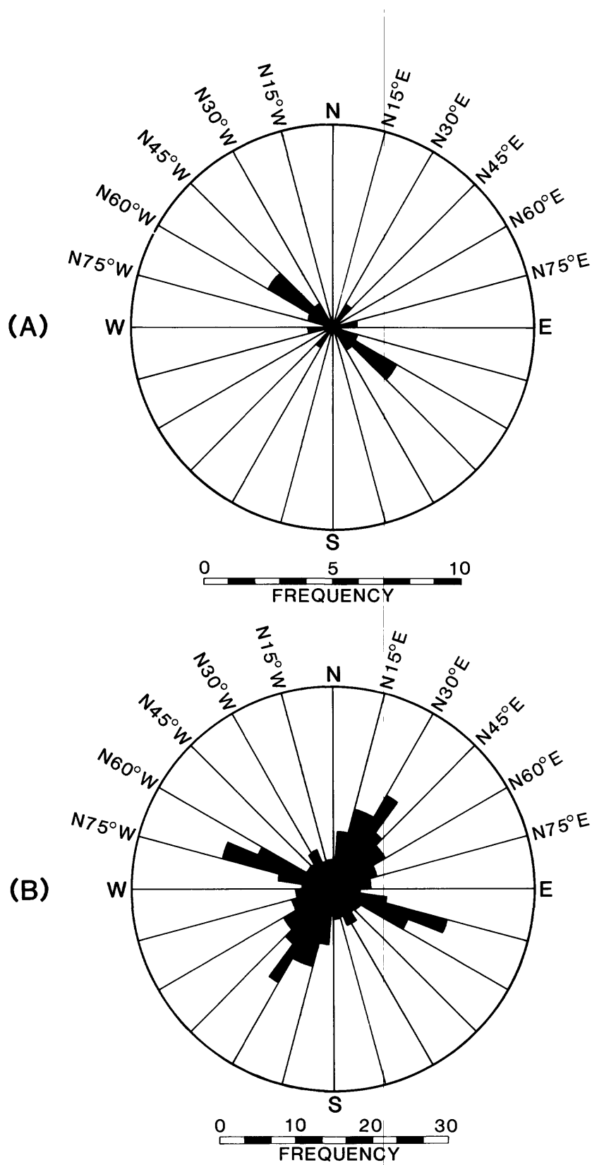
Figure 11.—Rose diagrams showing (A) frequency of orientation of the major component of transmissivity in the overburden aquifer and (B) frequency of orientation of bedrock joints in northeastern Monongalia County. (Modified from Bench and others, 1977, p. 18.)
