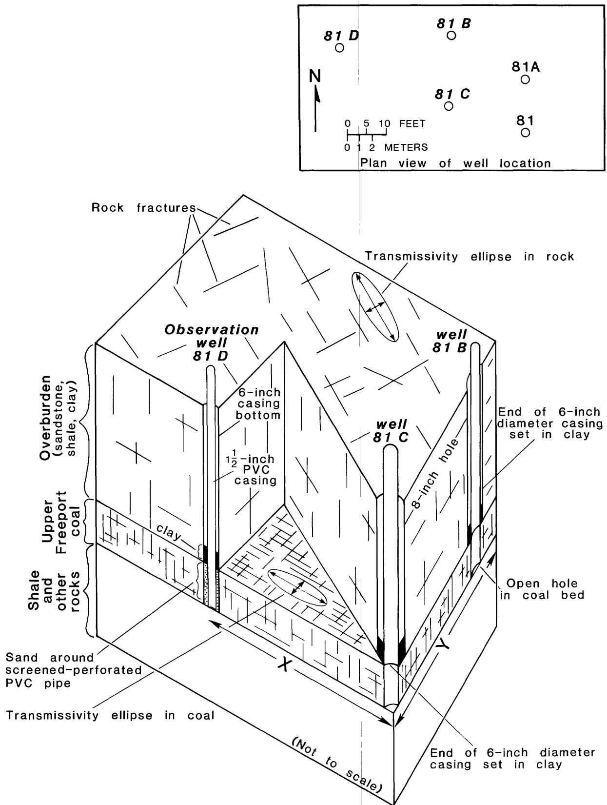
Figure 3.—Schematic diagram showing three test wells, their construction when testing the coal aquifer, and the orientation of maximum and minimum transmissivities for the overburden and coal aquifers. (The "X" line parallels the face cleat and the "Y" line nearly parallels the butt cleat in the coal.)
