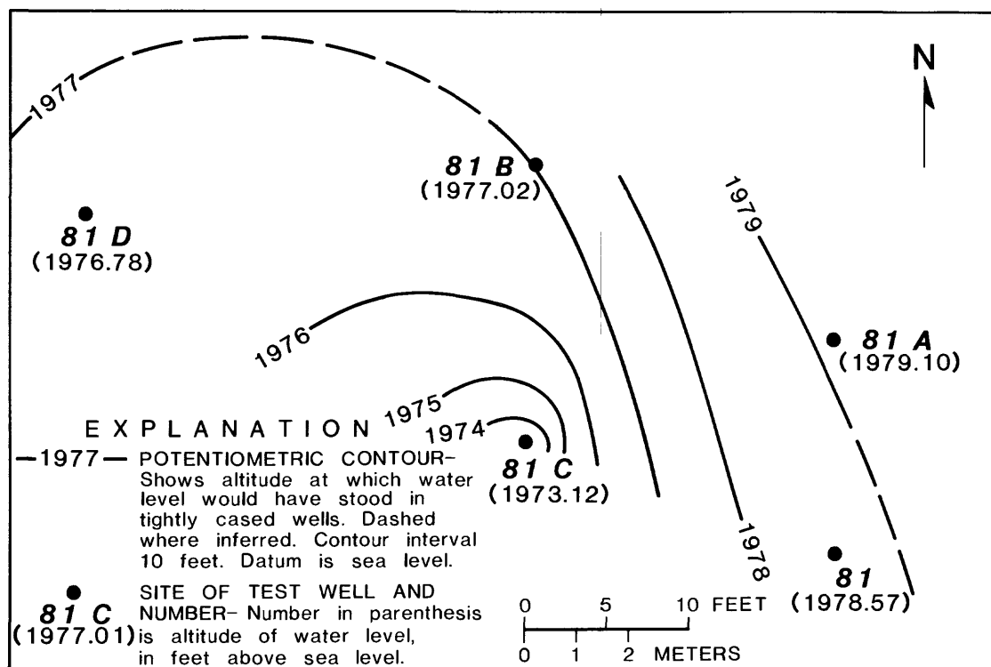
Figure 8.—Equipotential lines in bedrock above coal after 42 minutes of pumping well 81C at 1.0 gallons per minute.
