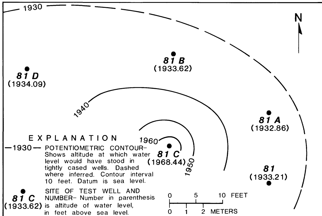
Figure 6.—Equipotential lines in coal aquifer 45 minutes after cessation of injection of water at well 81C at 0.9 gallons per minute for 115 minutes.
