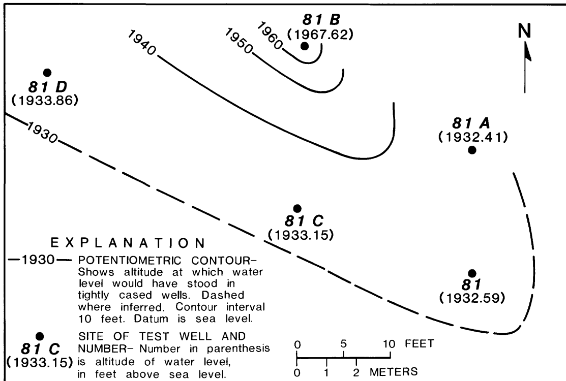
Figure 5.—Equipotential lines in coal aquifer after 110 minutes of injecting water at well 81B at 0.8 gallons per minute.
